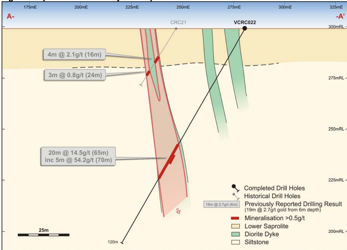
Figure 3 Apollo Drill Section. (See A-A' on Figure 2)
